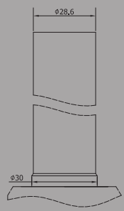
28.6 | 30 (1-1/8") STEERER | CROWN RACE
