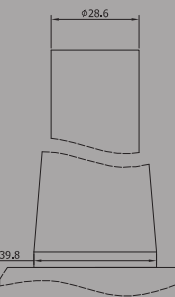
28.6 | 40 (1-1/8"-1.5") STEERER | CROWN RACE
